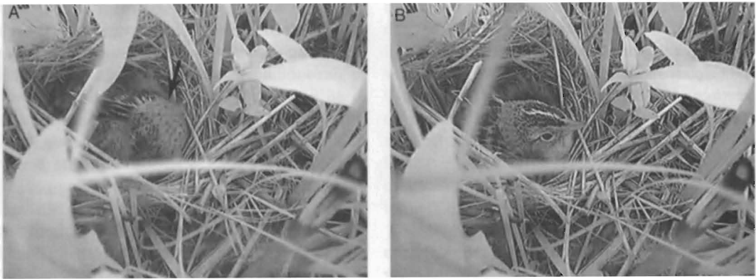
Figure 9.1. Typical postures of an adult passerine (a) in back sleep, with head turned to one side and bill tucked under scapular feathers (top of head indicated by arrow), and (b) vigilant while brooding young. These images of a Grasshopper Sparrow in southwestern Wisconsin were taken at 9 min and 6 min prior to sunrise, respectively.
