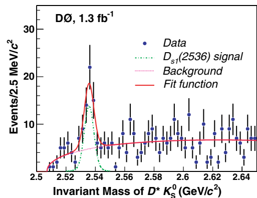
FIG. 2 (color online). Invariant mass of D^* K_S^0 with an associated muon. Shown is the result of the fit of the D^* K_S^0 mass with the function described in the text.
