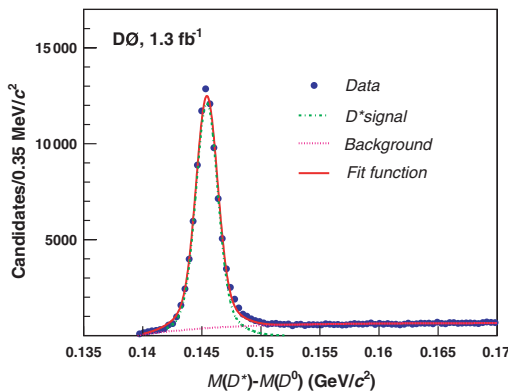
FIG. 1 (color online). The mass difference M(D^*) - M(D^0) for events with 1.8 < M(D^0) < 1.95 GeV/ c^2 and an associated muon. The number N_{D^* \mu} was defined as the number of signal events in the mass difference range of 0.142–0.149 GeV/ c^2 .
