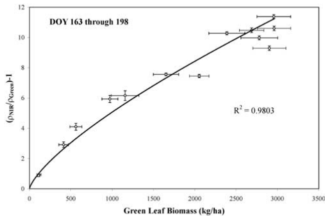
Figure 5. The index [(\rho_{\text{NIR}}/\rho_{\text{Green}}) - 1] plotted vs. green leaf biomass for the data between day of the year (DOY) 163 and 198 before tassels appeared.
