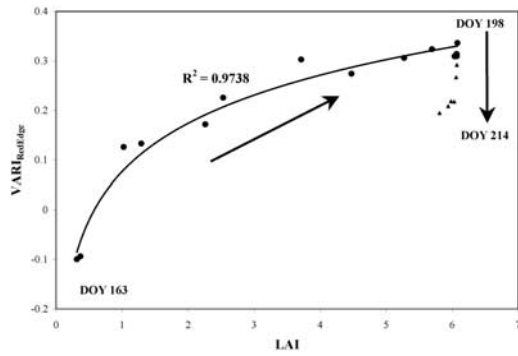
Figure 2. Visible Atmospherically Resistant Index ( VARI_{RedEdge} ) vs. LAI. The arrows show the direction of the progression of the growing season. Best-fit function was established between day of the year (DOY) 163 and 198 before tassels appeared.
