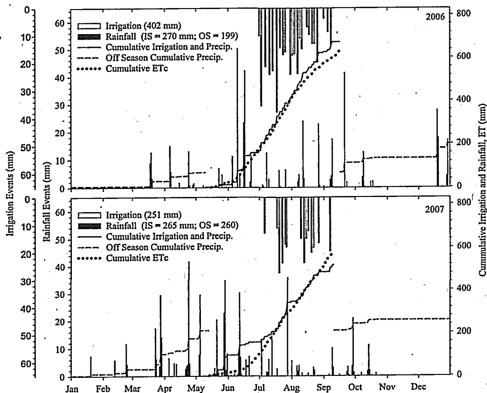
FIG. 1. Irrigation, precipitation, and evapotranspiration (ET) data from research area in 2006 and 2007. The ETc is the actual crop ET. During 2006 and 2007, ETc = ETw (ET assuming water is not limiting). The in-season (IS) period was from emergence to physiological maturity. The off-season (OS) period was the remaining time during the year.
