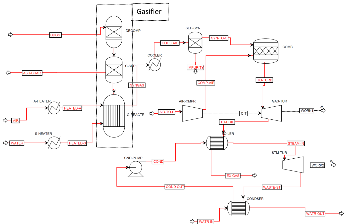
Figure 1. Process flow diagram of CHP generation from biomass gasification.
