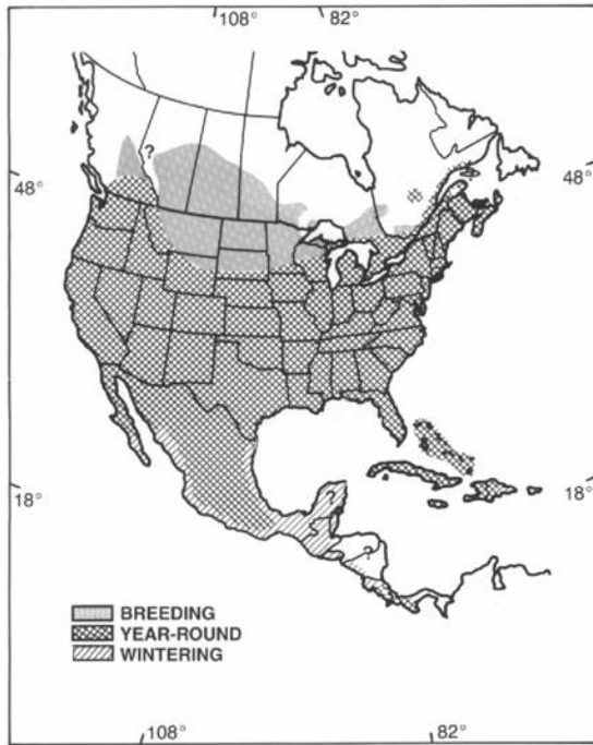
Fig. 1. Breeding and wintering ranges of the mourning dove (adapted from Mirarchi and Baskett 1994).
