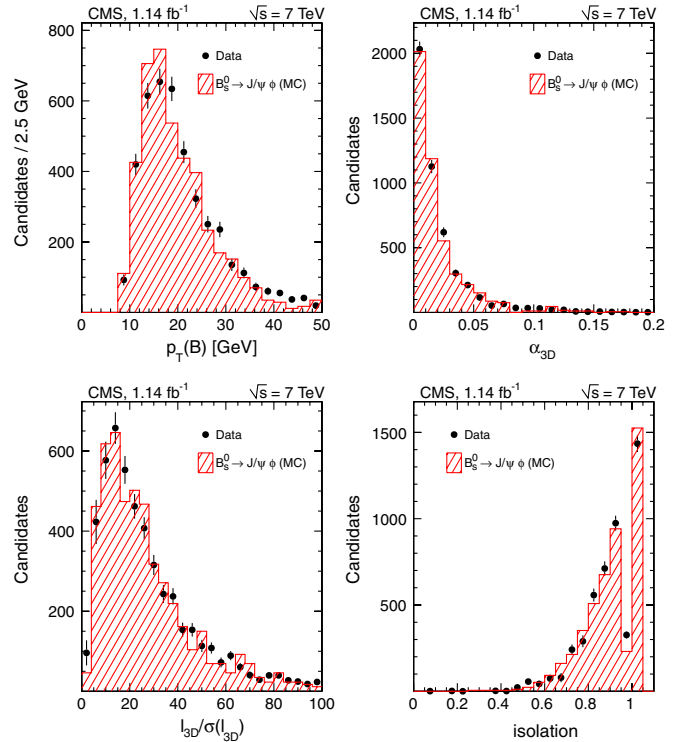
FIG. 2 (color online). Comparison of measured and simulated B_s^0 \rightarrow J/\psi \phi distributions, for the transverse momentum (top left), the 3D pointing angle (top right), the flight length significance (bottom left), and the isolation (bottom right). The MC histograms are normalized to the number of events in the data.
