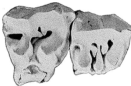
Fig. 3. Premolar 4 and molar 1, right upper, referred to Diceratherium loomisi , natural size. No. HC261.
