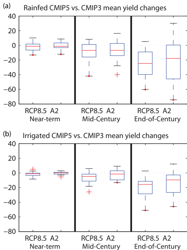
Fig. 7 Comparison of mean yield changes from three future time slices (near term, midcentury, and end of century relative to baseline mean) between the higher [CO_2] scenarios of 20 CMIP5 GCMs (RCP8.5) and 16 CMIP3 GCMs (A2) for (a) rainfed and (b) irrigated conditions.
