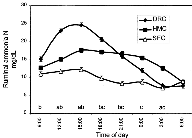
Figure 1. Effect of corn processing on ruminal ammonia concentration. Steers were fed at 0900. Treatment × time interaction ( P < 0.01 ). Differences among means within a sampling time are denoted by letters on the x-axis and the following footnotes. a Dry rolled corn (DRC) vs high moisture corn (HMC) ( P < 0.10 ). b DRC vs steam flaked corn (SFC) ( P < 0.10 ). c HMC vs SFC ( P < 0.10 ).
