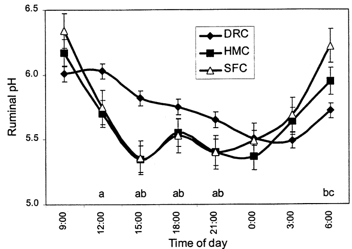
Figure 2. Effect of corn processing on ruminal pH. Steers were fed at 0900. Treatment × time interaction ( P < 0.01 ). Differences among means within a sampling time are denoted by letters on the x-axis and the following footnotes. a Dry rolled corn (DRC) vs high moisture corn (HMC) ( P < 0.10 ). b DRC vs steam flaked corn (SFC) ( P < 0.10 ). c High moisture corn (HMC) vs SFC ( P < 0.10 ).
