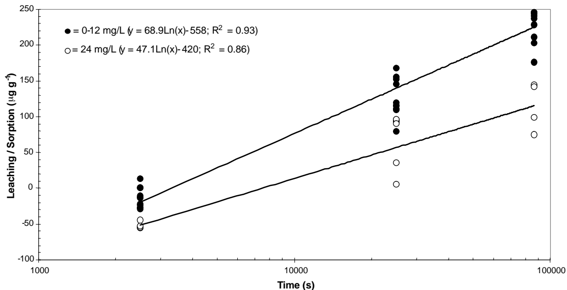
Figure 2. Leaching / sorption of \text{NH}_4\text{-N} by corn residue.
