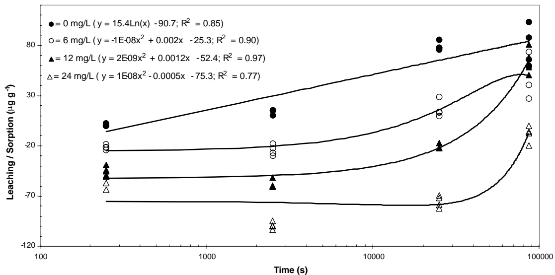
Figure 4. Leaching / sorption of \text{NH}_4\text{-N} by wheat residue.
