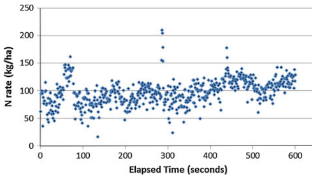
Fig. 6 Recommended N application rates for irrigated maize in Mexico using the “Drive-First” calibration approach at the V5 growth stage. Nitrogen rates were updated at 1 s intervals
