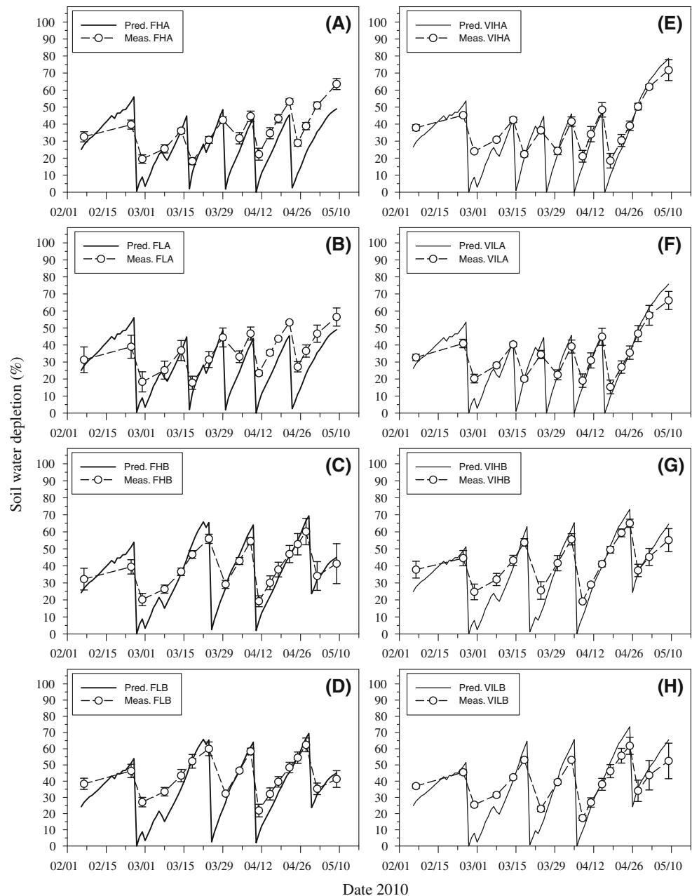
Fig. 8 Mean predicted and mean measured soil water depletion with time for sub-treatment FHA (a), FLA (b), FHB (c), FLB (d), VIHA (e), VILA (f), VIHIB (g), and VILB (h) in the 2010 experiment. Error bars about the measured means indicate the standard deviation
