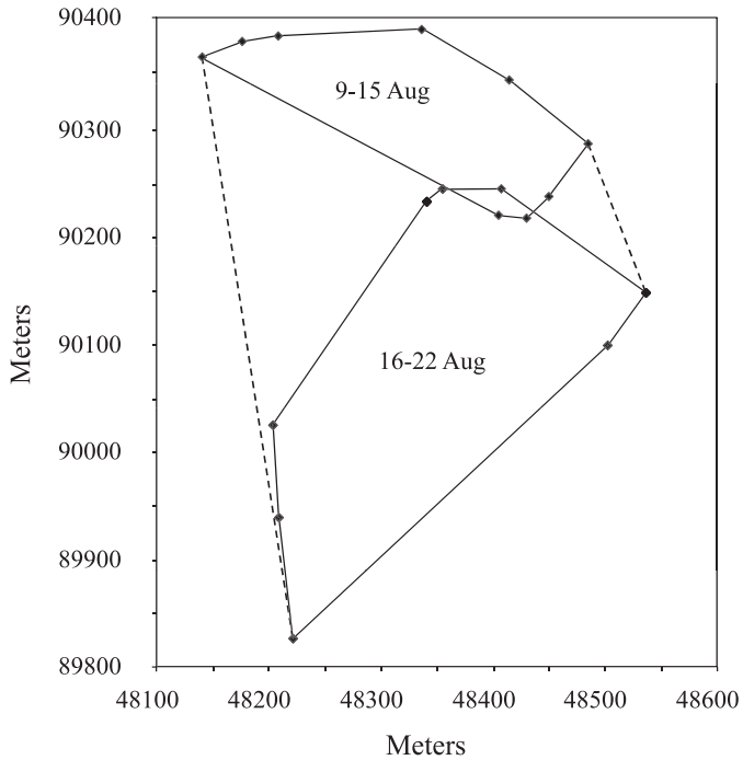
FIG. 2.—Activity area of radiotagged adult female black-footed ferret 08-83 during 9–22 August 1983. This 2-week, 13.63-ha area of activity is composed of 2 smaller activity areas from 9 to 15 August (2.97 ha) and 16 to 22 August (6.70 ha) that were used sequentially. Locations are shown using the Universal Transverse Mercator Zone 12 North.
