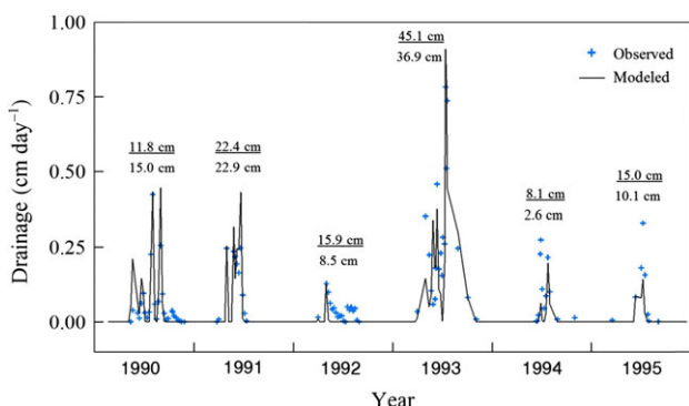
Figure 1. Weekly averaged, daily observed and RZWQM-predicted subsurface drainage rate from chisel-tilled plot 13 in Nashua, Iowa. The top number above each year is the measured annual flow volume, with the modeled volume beneath.
