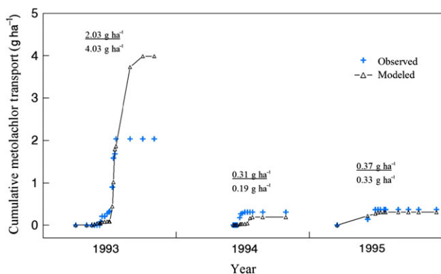
Figure 4. Cumulative metolachlor transport in subsurface drainage from chisel-tilled plot 13 in Nashua, Iowa. The top number above each year is the measured annual transport, with the modeled amount beneath.
