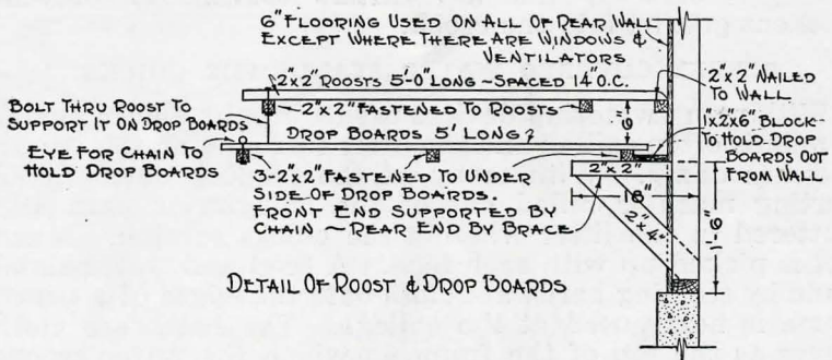
FIG. 12.—Cross section of plan of making drop boards and roosts movable without hinges.
