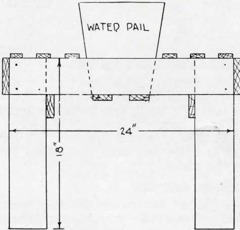
FIG. 9.—A stand for the water bucket.
