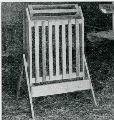
FIG. 16.—An inexpensive and movable rack for feeding alfalfa hay during the winter months.
