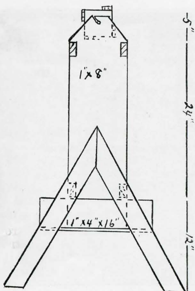
FIG. 17.—End view of a movable rack.
