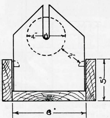
FIG. 4.—End view of large trough where a 4" brooder stove pipe or a gutter pipe is used for a reel. A lip for the edge of the trough is made by nailing quarter round to the inside of trough.
