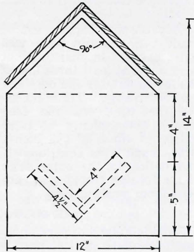
FIG. 5.—A wet mash feed trough protected by the inverted trough.
