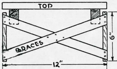
FIG. 10.—A low stand for a covered milk crock.
