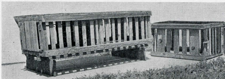
FIG. 22.—Combination marketing crate and broody coop to be placed under the trees. Made from box lumber.
