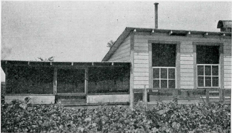
FIG. 20.—Suggested dimensions for building these hot weather roosting sheds are to be found in Extension Service circular No. 733.
