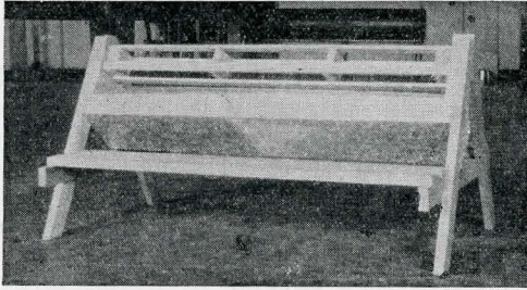
FIG. 1.—The "V" shaped feed trough made of various sizes of either metal or crating lumber \frac{3}{8} inch thick.
