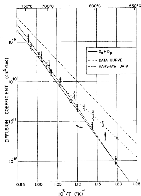
Fig. 3. Diffusion coefficient of Cl 36 in KCl containing Sr, as a function of temperature. - - - - -, Eq. (8) representing the Harshaw crystal data. ■, 237 ppm mole fraction strontium; ○, 469 ppm mole fraction strontium; —, calculated diffusion coefficients [see Eqs. (1), (2), and (7)]; ·····, anomalous behavior of 469-ppm Sr samples.
