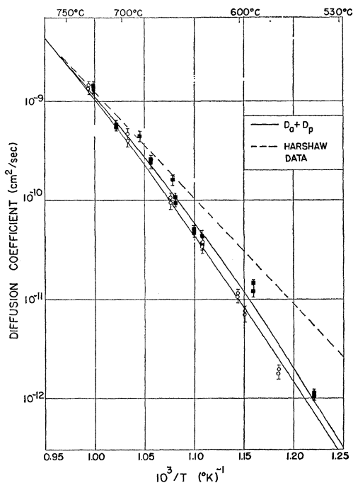
Fig. 2. Diffusion coefficient of Cl 36 in KCl containing Sr, as a function of temperature. - - - - -, Eq. (8) representing the Harshaw crystal data. ■, 21.0 ppm mole fraction strontium; O, 43.9 ppm mole fraction strontium; ———, calculated diffusion coefficients [see Eqs. (1), (2), and (7)].
