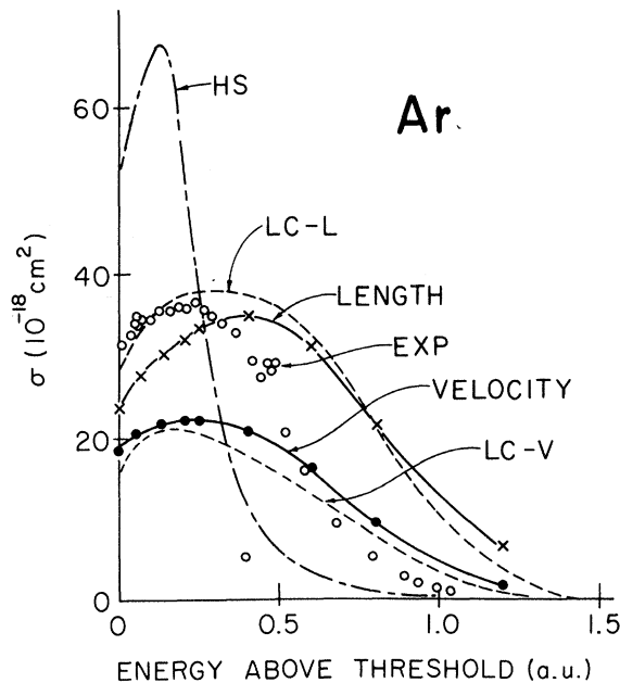
FIG. 1. Photoionization cross sections for the 3p shell in argon. Solid lines: meant to indicate the trend of the present results, which are the crosses (LENGTH) and dots (VELOCITY). LC-L and LC-V: Length and velocity results of L. Lipsky and J. W. Cooper (Ref. 10). HS: Herman-Skillman cross section. EXP: experimental results of J. A. R. Samson (Ref. 15).
