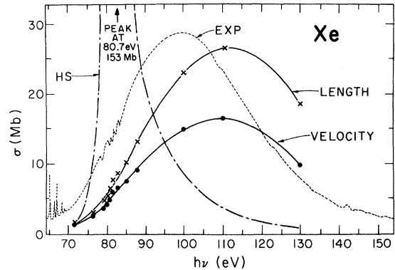
FIG. 2. Photoionization cross sections for the 4d shell in xenon. Solid lines: meant to indicate the trend of the present results, which are the crosses (LENGTH) and dots (VELOCITY). HS: Herman-Skillman cross section. EXP: experimental results of R. Haensel, G. Keitel, P. Schreiber, and C. Kunz (Ref. 16).
