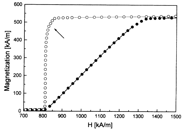
FIG. 2. Magnetization of \text{FeCl}_2 vs applied and internal fields H_a and H_i (solid and open circles, respectively) at T = 10 K. Rounding close to the paramagnetic saturation is indicated by an arrow.
