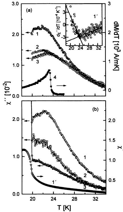
FIG. 3. Temperature dependence for \text{FeCl}_2 of (a) \chi'' at f=5 Hz and H_a=1592 kA/m (curve 3, circles), 1432 kA/m (curve 2, squares), and 955 kA/m (curve 1, triangles), dM/dT at H_a=0.8 kA/m (curve 4, filled squares), and d\chi''/dT (inset: curve 1', referring to curve 1), and (b) \chi'' at H_a=955 kA/m and f=10 Hz (curve 3, triangles), 1 Hz (curve 1, circles), and 0.1 Hz (curve 2, squares) and \chi' at H_a=955 kA/m and f=1 Hz (curve 1').
