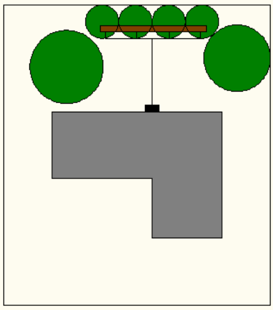
Note: The grey area is the house. The black box attached to the house is the tipper box, the brown box under the small trees is a mulch basin. Each black line represents 2" (50.8 mm) PVC pipe. From: (Gardels 2011)
