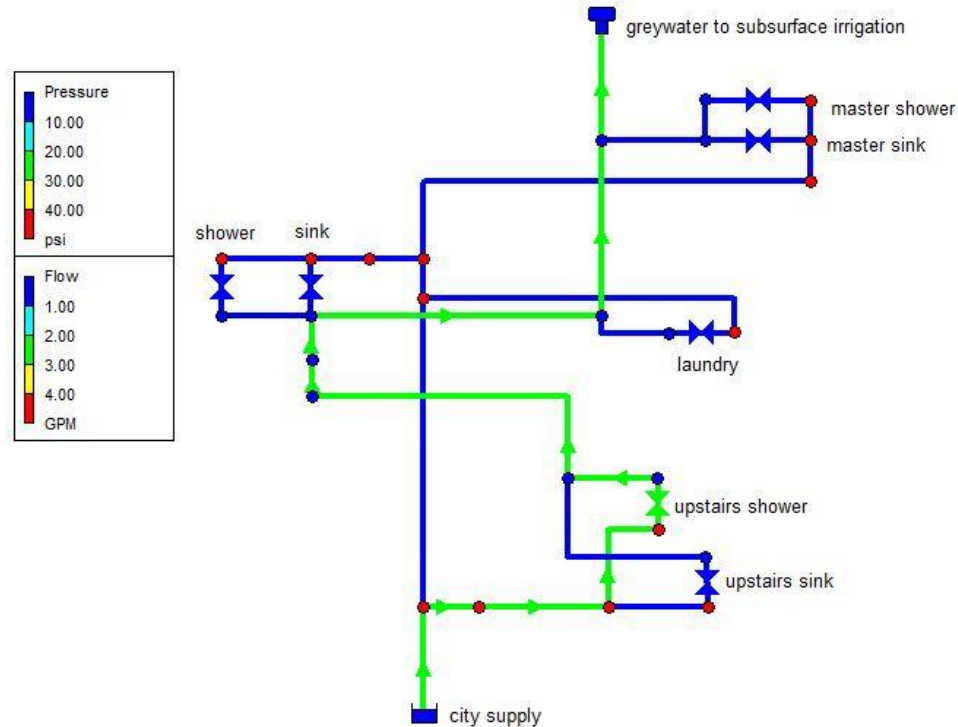
Figure 3.6 Screenshot of the Simple Greywater Collection Scenario in EPANET 2.
