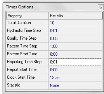
Figure 3. “Time Options” menu in EPANET.
