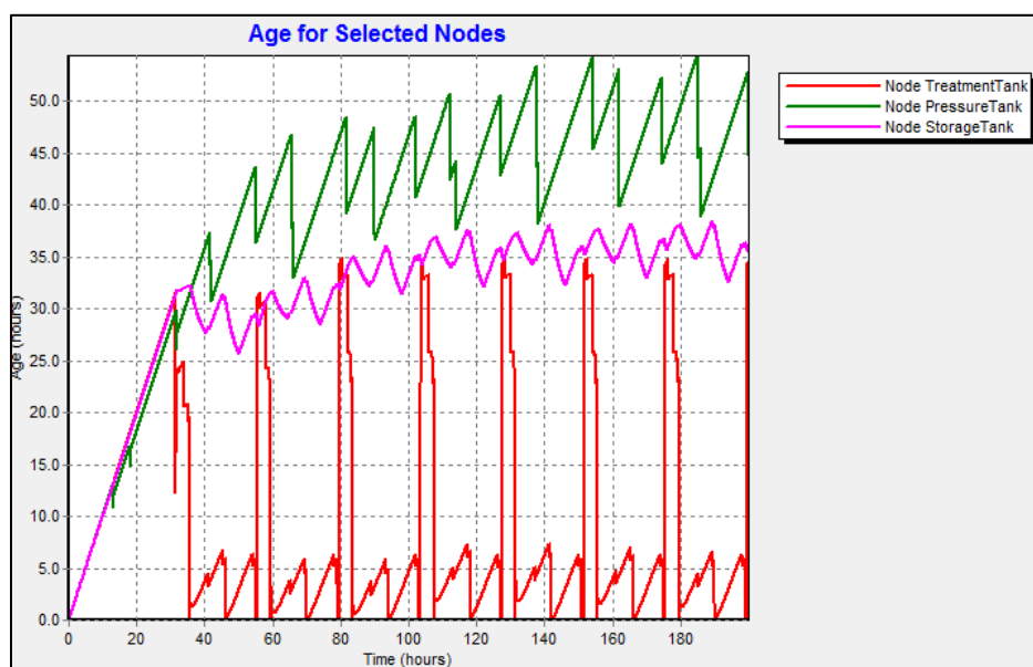
Figure 3.9 Maximum Water Age for the Complex Greywater System with Treatment.
