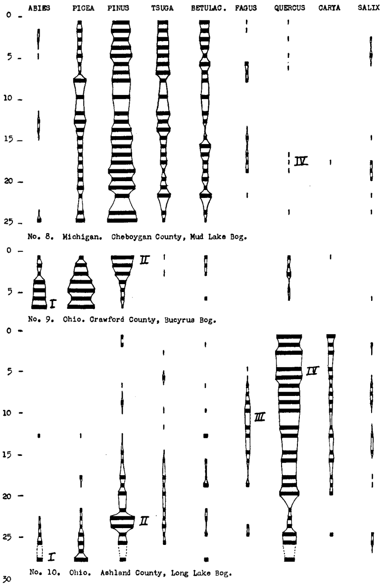
FIG. 4.—Pollen profiles of important forest components, bogs 8-10
