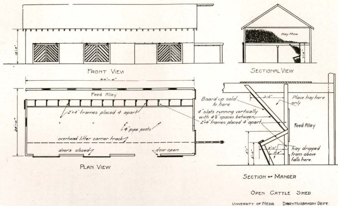
FIG. 13—PLAN OF OPEN SHED IN USE AT THE UNIVERSITY OF NEBRASKA Dry cows and heifers may be housed and fed roughage in this shed with the expenditure of but little labor. This arrangement was also found of advantage in summer for feeding soiling crops and providing shade for cows being tested for advanced registry. The large doors on the south side are closed only during the coldest weather.
