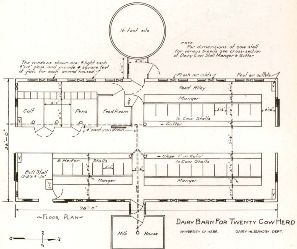
FIG. 12—SUGGESTED ARRANGEMENT OF FIRST FLOOR IN BARN OF TWENTY-COW HERD
