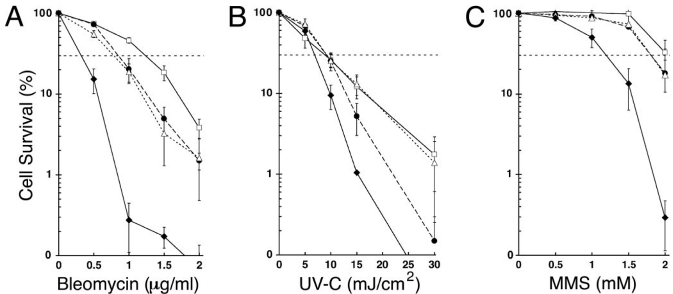
Figure 4. Effect of DNA-damaging agents on the survival of the mutant and wild-type strains. Each graph point represents the mean ( \pm standard error) of nine replicates (three independent experiments). Where the error bars are not visible, they are smaller than the symbols. The dashed horizontal lines indicate 30% cell survival. Symbols: \square , wild-type CC-124; \bullet , Mut-9; \triangle , Mut-11; \blacklozenge , Mut-9 Mut-11. (A) Survival of the mutants and wild-type C. reinhardtii grown on TAP medium containing increasing concentrations of bleomycin. (B) Survival of the mutants and wild-type C. reinhardtii exposed to increasing doses of UV-C irradiation under nonphotoreactivating conditions. (C) Survival of the mutants and wild-type C. reinhardtii grown on TAP medium containing increasing concentrations of methyl methanesulfonate (MMS).
