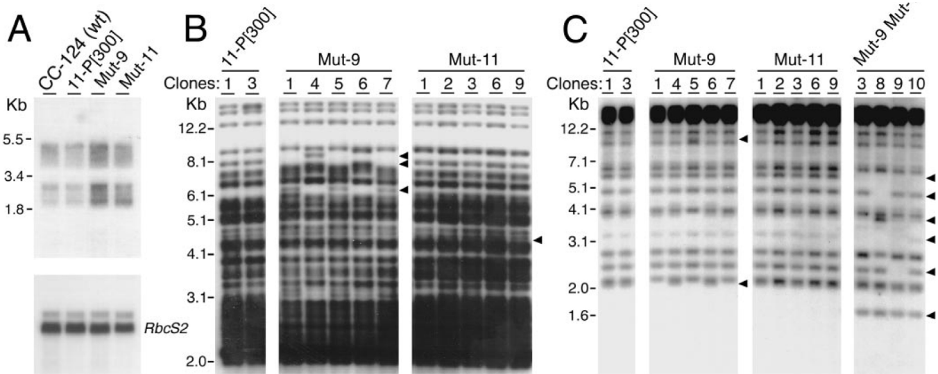
Figure 2. Reactivation of a retroelement, TOC1 , and a DNA transposon, Gulliver , in the mutant strains. Abbreviations are as in the legend to Figure 1. (A) Northern blot of total RNA probed sequentially for TOC1 (Upper) to examine transcript levels and for RbcS2 (Lower) to test for equal loading of the lanes. (B) Southern blot analysis of TOC1 transposition. Genomic DNA from parallel subcultures (Clones) of the indicated strains was digested with HincII and probed for TOC1 . The arrowheads indicate new fragments in the subclones of Mut-9 and Mut-11. (C) Southern blot analysis of Gulliver transposition. Total cell DNA from parallel subcultures (Clones) of the indicated strains was digested with HindIII and probed for Gulliver . The arrowheads indicate missing or new fragments in the subclones of Mut-9 and Mut-9 Mut-11. Although only two subclones are shown for 11-P[300], we did not detect mobilization of either TOC1 or Gulliver in 10 parallel subcultures grown under the same conditions as the mutant strains.
