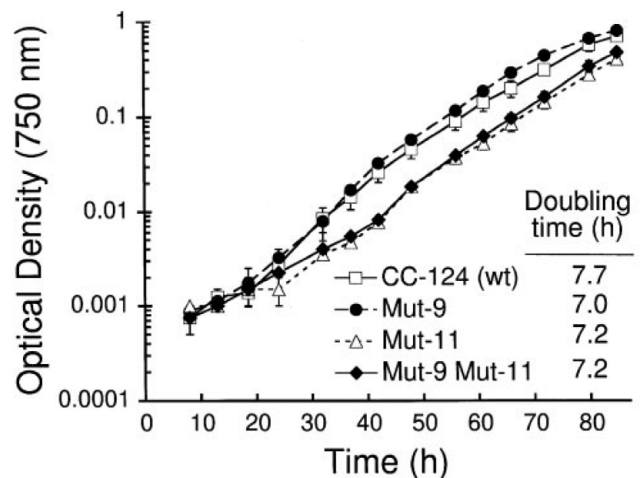
Figure 3. Photoheterotrophic growth of the mutant and wild-type strains. Abbreviations are as in the legend to Figure 1. Each time point represents the mean ( \pm standard error) of six replicates (three independent experiments). Where the error bars are not visible, they are smaller than the symbols. The exponential phase of the growth curve was used to calculate doubling times. Even though all strains show similar doubling times, Mut-11 and Mut-9 Mut-11 took considerably longer to reach exponential growth (represented by a linear increase in optical density in the semilogarithmic scale).
