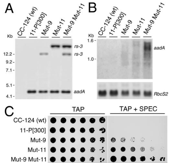
Figure 1. Expression of the RbcS2::aadA::RbcS2 transgene is reactivated in the mutant strains. (A) Southern blot analysis of the wild-type untransformed strain (CC-124), the silenced parental strain (11-P[300]), the mutant strains (Mut-9 and Mut-11), and a double mutant strain (Mut-9 Mut-11). Total cell DNA was digested with HindIII and hybridized to the pBluescript vector backbone, which is common to the plasmids containing the chimeric aadA transgene or the tagging rs-3 gene. The fragments corresponding to the transgene ( aadA ) or the insertional mutagen ( rs-3 ) are indicated. (B) Northern blot analysis of the strains described above. Total cell RNA was isolated from each strain, separated under denaturing conditions, and hybridized to the aadA coding sequence (Upper). The same blot was reprobed with the coding sequence of RbcS2 as a control for equal loading of the lanes (Lower). The faint transcript seen above RbcS2 corresponds to the RbcS1 gene (11). (C) Growth and survival on TAP medium or on TAP medium containing spectinomycin (TAP + SPEC) of the indicated strains. Five-fold serial dilutions of cells, starting with 1 \times 10^5 cells on the left, were spotted on each plate and incubated for 15 days (12).
