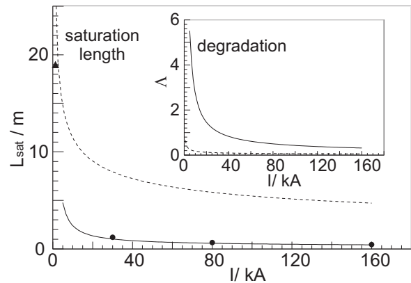
FIG. 2: Saturation lengths (Eq. 3) and (inset) degradation factor \Lambda as a function of electron beam current I : DESY's FLASH (dashed curve, triangle) and the table-top VUV scenario (solid line). The circles denote specific GENESIS runs.
