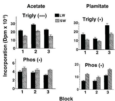
Figure 2. Amount of radiolabeled [ 1\text{-}^{14}\text{C} ]acetate or [ 1\text{-}^{14}\text{C} ]palmitic acid incorporated into triglyceride or phospholipid in LW(f) or SW G. firmus on day 5 of adulthood. Trigly, triglyceride; Phos, phospholipid. Block refers to independent selection trial (see Materials and Methods ). The asterisks in parentheses indicate results of paired t tests (***, P < 0.005 ; *, P < 0.05 ). Values in all panels are means ( \pm SEM) based on 20–28 individuals. On day 0, mean triglyceride or phospholipid dpm (from [ 1\text{-}^{14}\text{C} ]acetate) did not differ significantly between morphs within any block ( P > 0.1 for all ANOVAs) or across blocks ( P > 0.1 for paired t tests). Grand mean dpm (means across the three blocks) are as follows: triglyceride, 9,606 \pm 1,814 [LW(f)] and 9,328 \pm 1,861 (SW); phospholipid, 3,030 \pm 139 [LW(f)] and 2,861 \pm 188 (SW).
