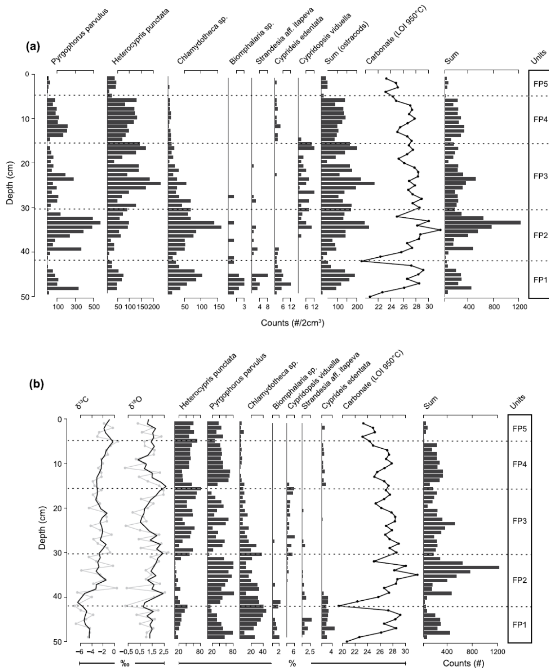
Figure 4. Ostracod and gastropod fauna of Freshwater Pond sediment core FP2 (a) absolute fossil counts (#) for each taxon per 2 cm 3 of sediment and the corresponding curves for the total sum of ostracod valves, carbonate content and the total sum for all micro- and macrofossil counts. The biostratigraphic units FP1-5 are delimited by boundaries defined by the absence of the freshwater gastropod Pyrgophorus parvulus . (b) Stable carbon and oxygen isotope measurements determined from fossil valves of the ostracod Heterocypris punctata compared with the relative abundance of selected ostracod and gastropod taxa, the carbonate content of sediment core FP2 and the total sum of all micro- and macrofossil counts. Light gray lines represent the original stable isotope measurements and the black line is a 5-point running mean of the isotope time series.
