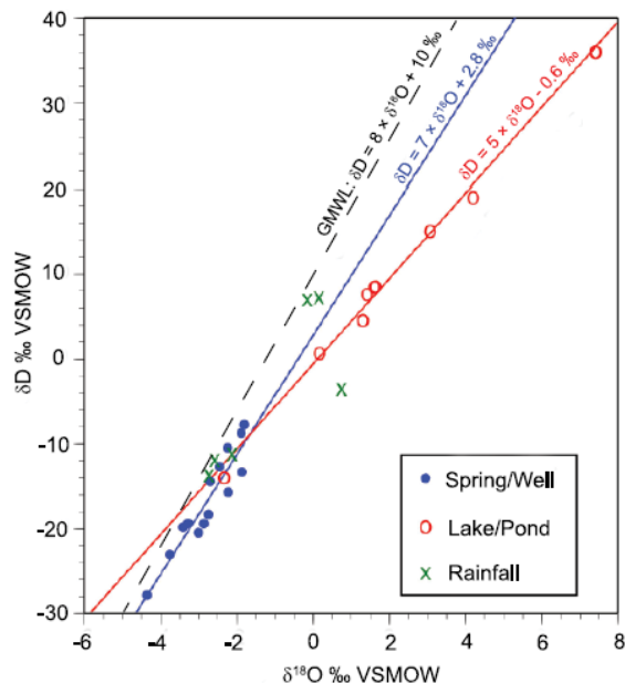
Figure 2. Plot of the stable isotope composition of ground water, precipitation and lake water in Barbuda collected on several occasions in May 2012 and between April and October 2013. Note the linear least squares regression lines for spring and lake waters have a lower gradient and fall below that of the Global Meteoric Water Line (GMWL) suggesting evaporative enrichment of the collected samples. Groundwater and rainfall samples were recovered from man-made wells and rainfall collectors on the Highlands Plateau. Lake water samples were collected from Freshwater Pond.
