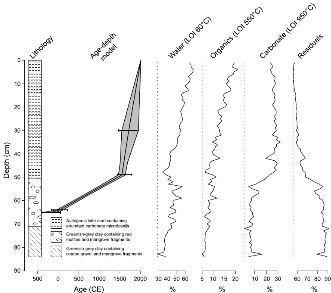
Figure 3. Sediment stratigraphy, age-depth model and the corresponding water, organic matter, carbonate and residual curves determined by loss-on-ignition for sediment core FP2 from Freshwater Pond, Barbuda.
