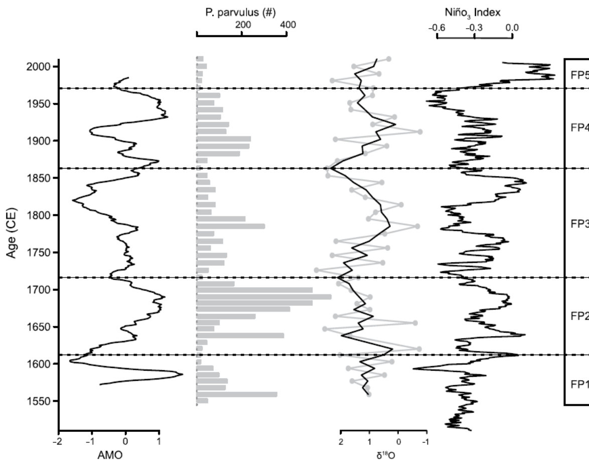
Figure 5. Comparisons between the tree-ring-based reconstructions of the Atlantic Multidecadal Oscillation (AMO) of Gray et al. (2004) and El Niño Southern Oscillation (ENSO) of Li et al. (2013) and counts of the freshwater gastropod Pyrgophorus parvulus (Guilding, 1828) and the oxygen isotope determinations of ostracod calcite of Heterocypris punctata (Keyser, 1975) for the period 1500 CE–present.
