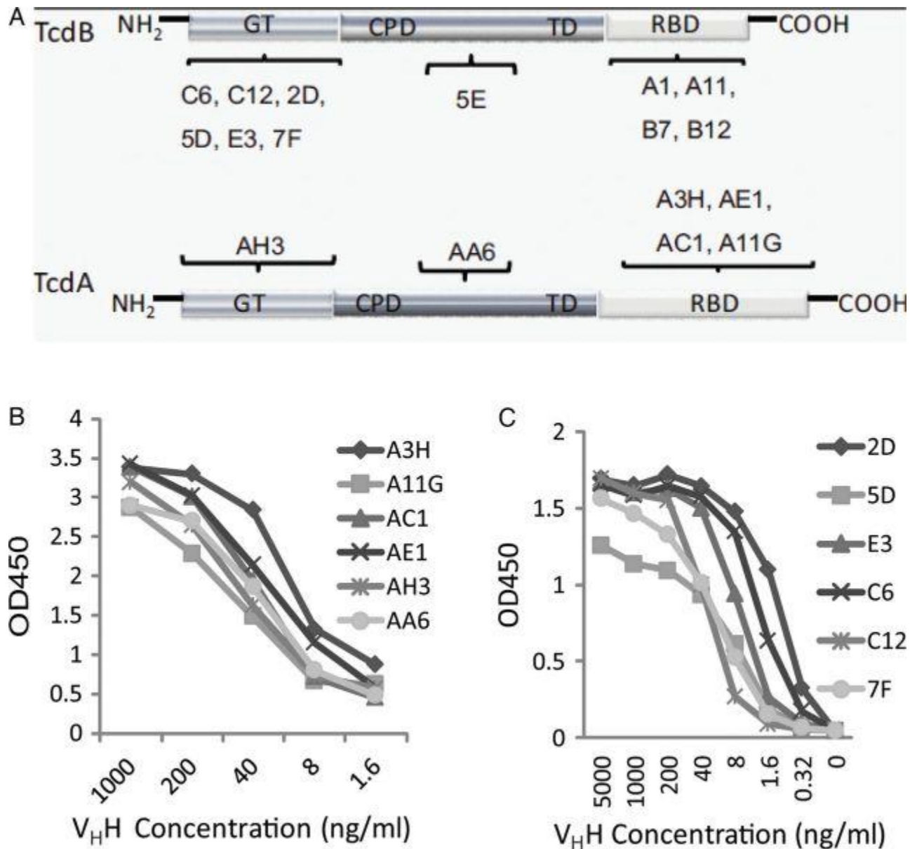
Figure 1. Binding of specific heavy-chain-only antibody (V H H) to TcdA and TcdB. A , Diagram illustrates specific binding of individual V H Hs to the glucosyltransferase domain (GTD), cysteine protease domain (CPD), translocation domain (TD), or receptor-binding domain (RBD) in TcdA or TcdB. B and C , Enzyme-linked immunosorbent assay analysis of serially diluted anti-TcdA ( B ) or anti-TcdB ( C ) V H Hs in microtiter plates coated with 0.5 μg/mL of TcdA or TcdB, respectively.
