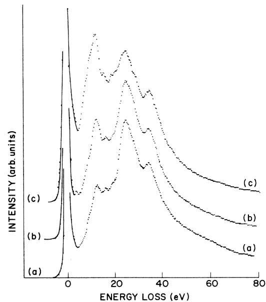
FIG. 2. (a), (b), and (c) are electron-energy-loss spectra obtained from three spots 1500, 1000, and 500 Å from a thin edge of a pinhole. Note the increase of the 13.5 eV intensity toward the edge of the pinhole.
