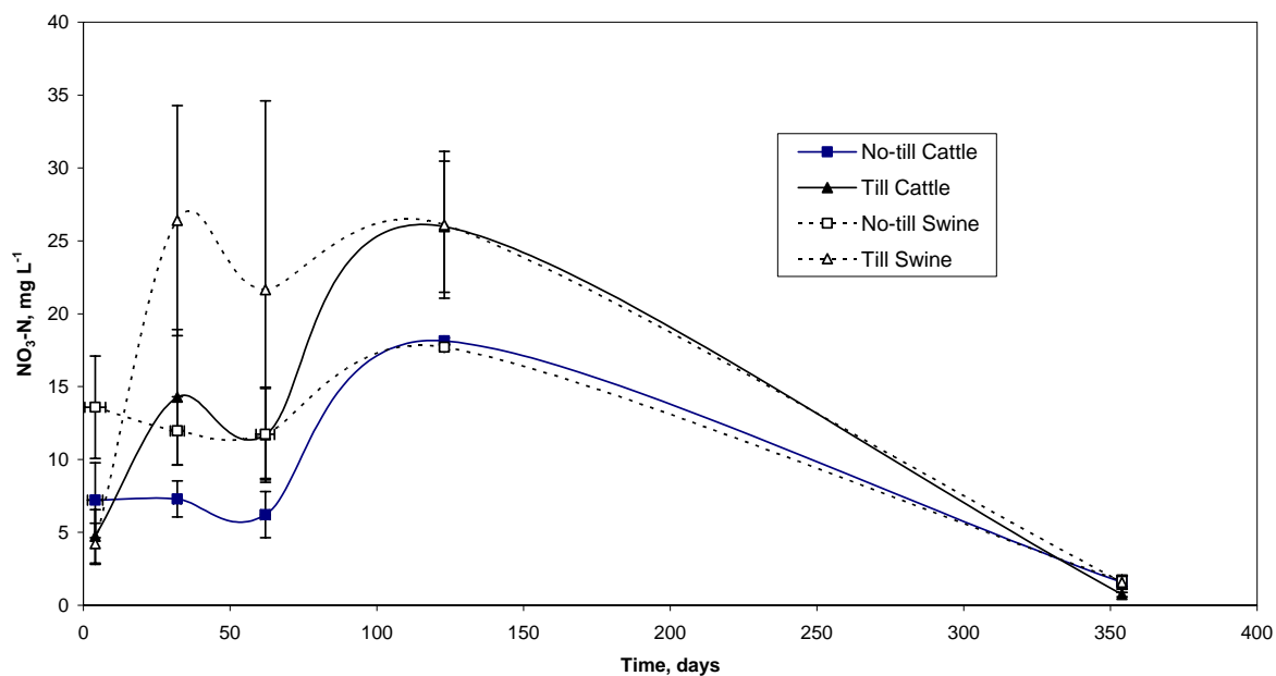
Figure 3a. \text{NO}_3\text{-N} concentrations of runoff versus time since manure application for the experimental treatments. Vertical bars represent one standard deviation of the mean value.
