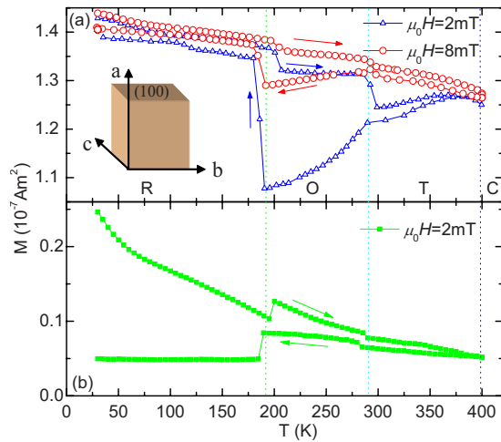
FIG. 1. (Color online) (a) Variation of the Fe film in-plane magnetization, M_{\parallel} , with temperature, T , at magnetic fields, \mu_0H = 2 mT (triangles) and 8 mT (circles). The arrows point to the direction of temperature scans. Letters R, O, T, and C denote the rhombohedral, orthorhombic, tetragonal, and cubic states of BaTiO 3 single-crystal substrate, respectively. The dotted lines are the boundaries between respective transitions. The inset depicts a representative BTO unit cell with reference axes. (b) M_{\perp} vs T curves at \mu_0H = 2 mT.
