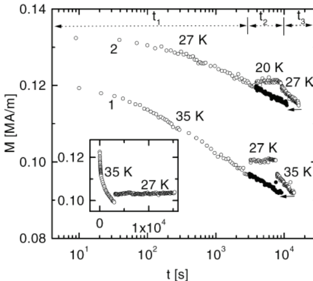
Figure 2. Relaxation curves of M^{\text{TRM}} after field cooling with \mu_0 H = 0.4 mT at (1) T_m = 35 K ( t < 3000 s), 27 K ( 3000 < t < 8000 s) and 35 K ( 8000 < t < 14\,000 s) and (2) T_m = 27 K ( t < 4000 s), 20 K ( 4000 < t < 9000 s) and 27 K ( 9000 < t < 17\,000 s). The data referring to the last time intervals have been replotted against t - 8000 s as solid circles as indicated by arrows. The inset shows the relaxation cycle at T_m = 35 K ( t < 3000 s) followed by a prolonged period ( 3000 < t < 15000 s) at 27 K.
