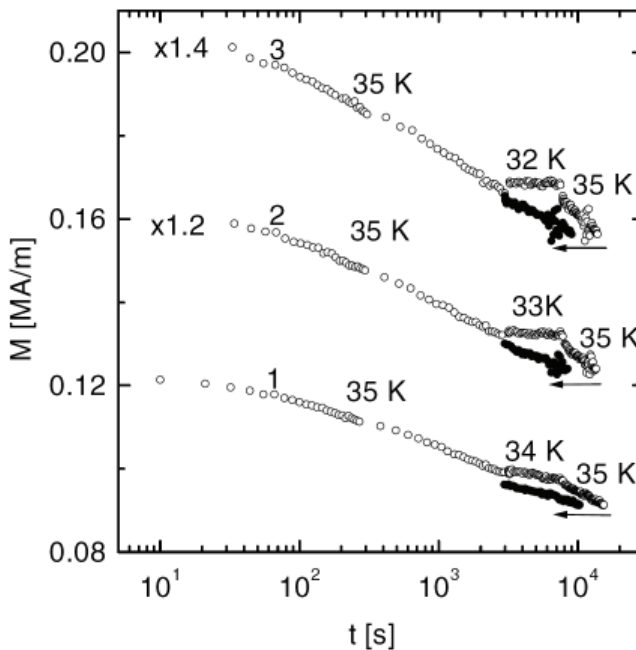
Figure 4. Relaxation curves of M^{\text{TRM}} after field cooling with \mu_0 H = 0.4\text{ mT} at (1) T_m = 35\text{ K} ( t < 3,000\text{ s} ), 34\text{ K} ( 3,000 < t < 8,000\text{ s} ) and 35\text{ K} ( 8,000 < t < 14,000\text{ s} ), (2) T_m = 35\text{ K} ( t < 3,000\text{ s} ), 33\text{ K} ( 3,000 < t < 8,000\text{ s} ) and 35\text{ K} ( 8,000 < t < 14,000\text{ s} ) and (3) T_m = 35\text{ K} ( t < 3,000\text{ s} ), 32\text{ K} ( 3,000 < t < 8,000\text{ s} ) and 35\text{ K} ( 8,000 < t < 14,000\text{ s} ). All data sets obtained within 8,000 < t < 14,000\text{ s} have been replotted against t - 5,000\text{ s} (solid circles).
