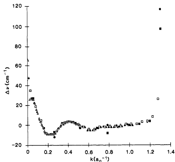
Figure 3. Dependency of the frequency shift vs wavevector behavior upon the number of atoms in a chain (all chains having the same number): 11 (●), 21 (○), 51 (■), 101 (□), 201 (▲), and 401 (△).
