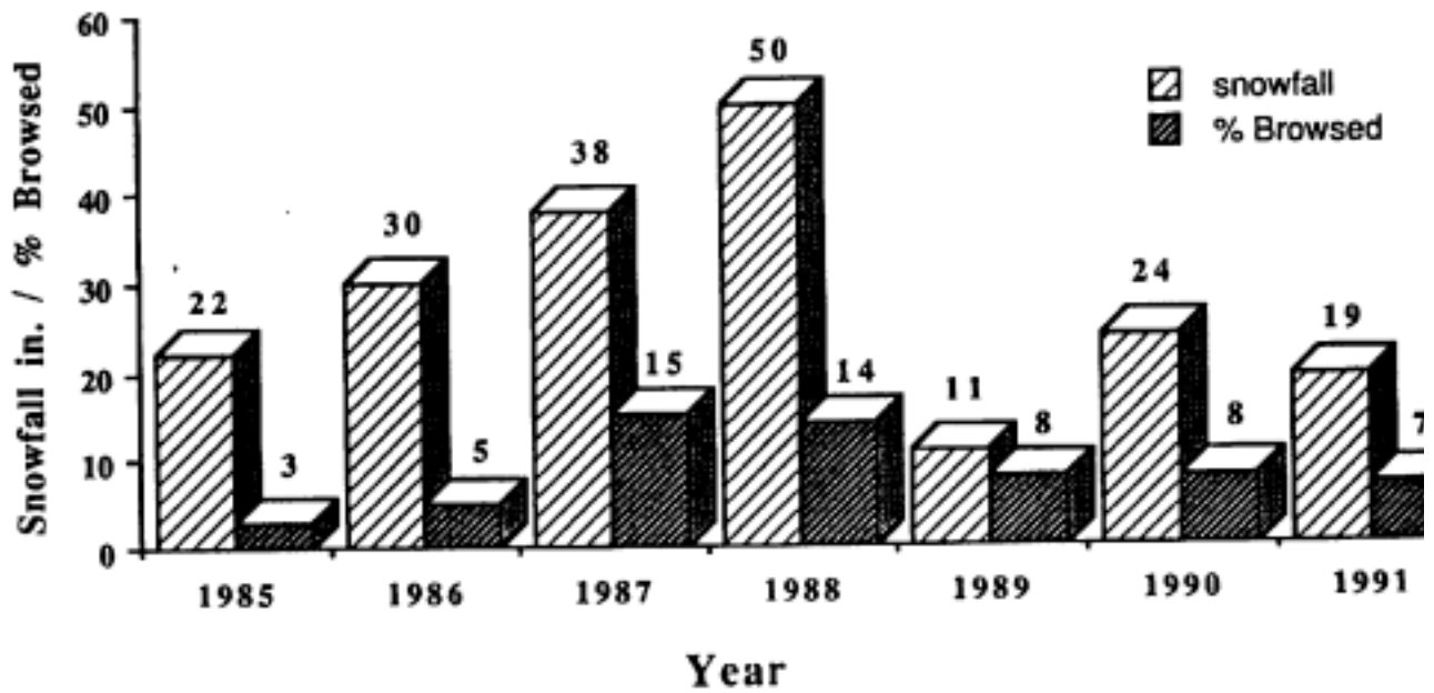
Fig. 3. Total winter snowfall (inches) versus the proportion of total stems browsed at Cary Arboretum, Dutchess County, New York, during 1985-91.
