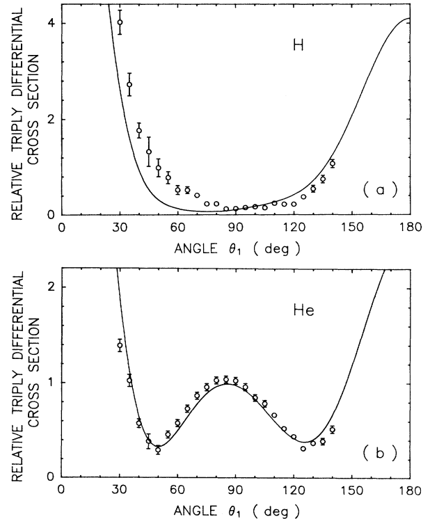
FIG. 2. Relative triply differential cross sections [cf. Eq. (7)] for \theta_{12} = \pi , \frac{1}{2}k_1^2 = 3.5 eV, and \frac{1}{2}k_2^2 = 0.5 eV for (a) H and (b) He targets. Solid curves: Present results including the effective electron-electron screening potential [cf. Eq. (5)]. Open circles: Experimental results of Schlemmer et al. [4].
