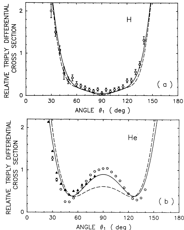
FIG. 1. Relative triply differential cross sections [cf. Eq. (7)] for \theta_{12} = \pi and \frac{1}{2} k_1^2 = \frac{1}{2} k_2^2 = 2 eV for (a) H and (b) He targets. Solid (dashed) curves: Present results including (not including) the effective screening potential [cf. Eq. (5)]. Open circles: Experimental results of Schlemmer et al. [4]. Solid triangles: Experimental results of Selles, Huetz, and Mazeau [3].
