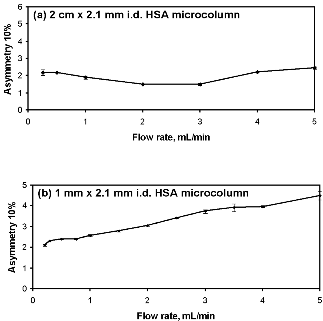
Figure 5. Measured peak asymmetry at tenth height width for 5 \mu L injections of 20 \mu M R -warfarin onto HSA microcolumns with lengths of (a) 2 cm or (b) 1 mm and an inner diameter of 2.1 mm. Other experimental conditions are given in the text. The error bars represent a range of \pm 1 S.D. of the mean.
