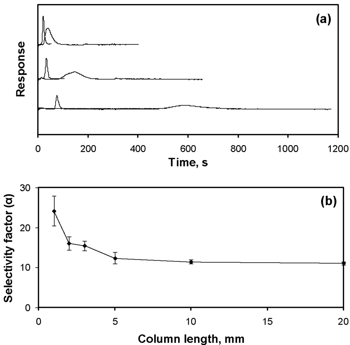
Figure 3. (a) Typical chromatograms obtained for R -warfarin and L -tryptophan and (b) the resulting selectivity factors determined R -warfarin versus L -tryptophan for HSA microcolumns. The results in (a) were generated using HSA microcolumns with lengths of 20, 5 or 1 mm and an inner diameter of 2.1 mm. Other experimental conditions are given in the text. The error bars represent a range of \pm 1 S.D. of the mean.
