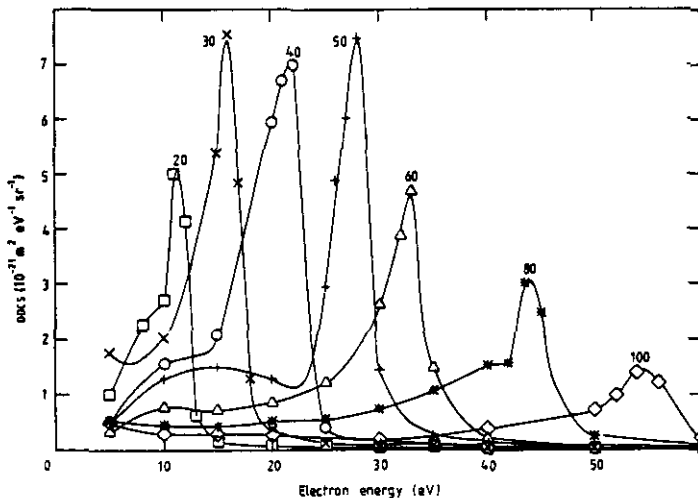
Figure 2. Doubly-differential cross sections in energy for 0^\circ emission of electrons in H^+He collisions at proton energies between 20 keV and 100 keV [33]. An apparent mid-velocity secondary maximum, evident between 40 and 60 keV, disappears at higher energies, and, if present, is not resolved at lower ones. See also refs. 7,8, and 18.
