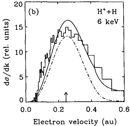
Figure 1. Relative electron yield vs. electron velocity for 6 keV H^+ + H collisions. Projectile velocity divided by two is indicated by the arrow. The dash-dot curve indicates the theoretical prediction for the saddle-point electron contribution; the solid curve is the total yield prediction, fitted with one height parameter to the experimental results. Data and theory of ref. [20].
