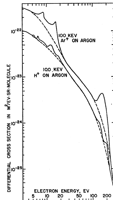
FIG. 1. Doubly-differential cross-sections for ejection of electrons from argon by protons and argon ions at 100 keV. Electrons are detected at 160^\circ from the beam direction. Resolution varies from 0.5 eV at 3 eV energy to 12 eV at 300 eV.
