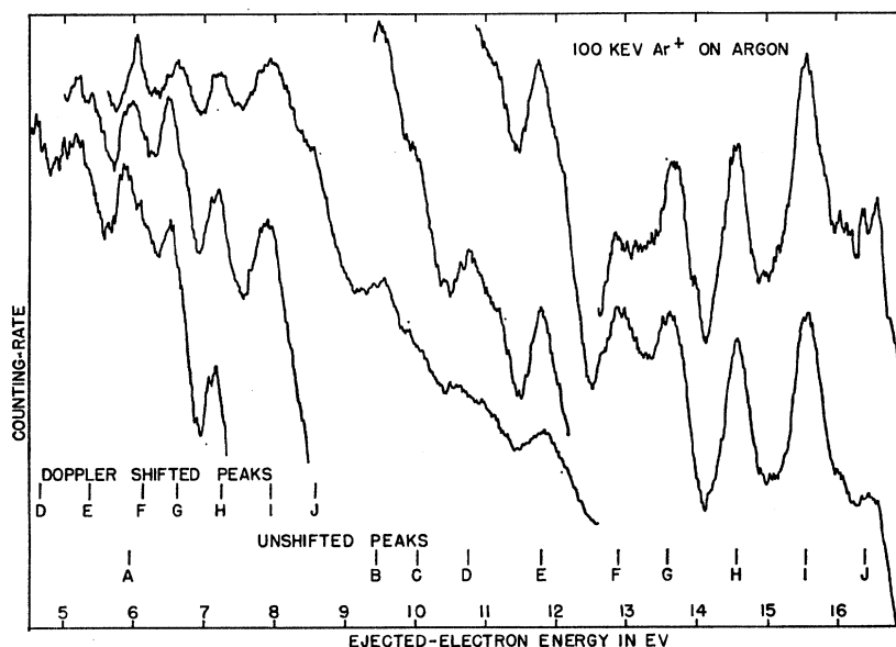
FIG. 2. Energy spectrum of electrons from 100-keV \text{Ar}^+ -Ar collisions. Resolution about 0.2 eV.
