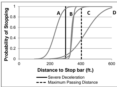
Fig. 7 – Hypothetical probability of stopping curves
