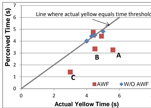
Fig. 8 – Comparison between actual and perceived yellow lengths
