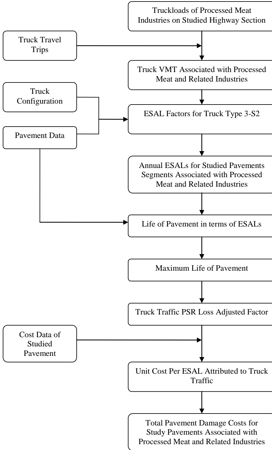
Fig. 3.2 Flowchart of Pavement Damage Cost Analysis Procedure
