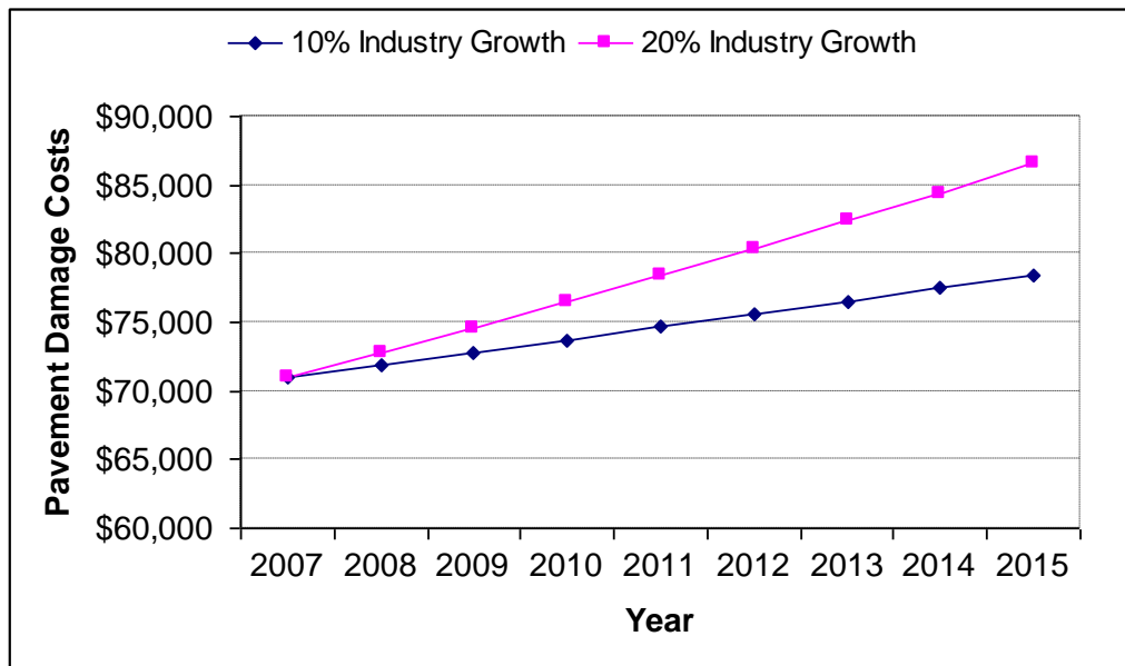
Fig. 3.5 Projected Future Annual Pavement Damage Costs Associated with Meat Processed and Related Industries on the Studied Highway Section
