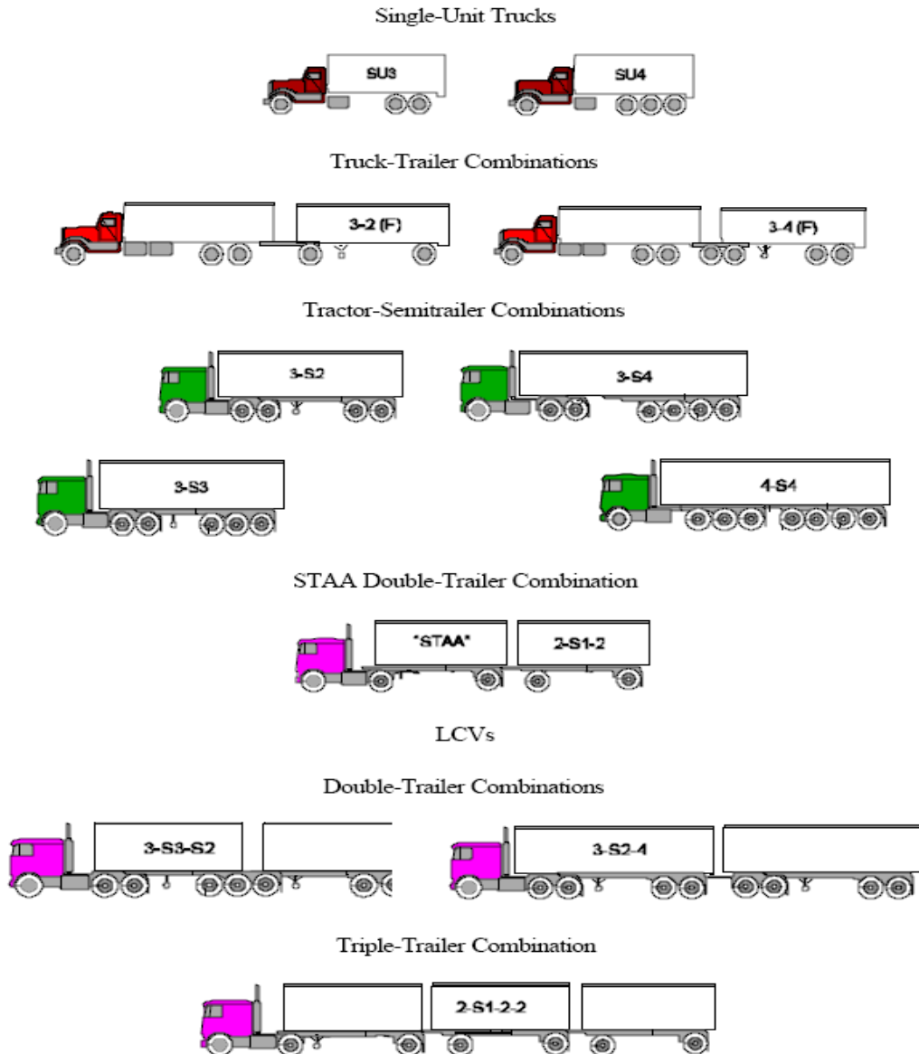
Fig. 5.1 Illustrative Truck Fleet Configuration
