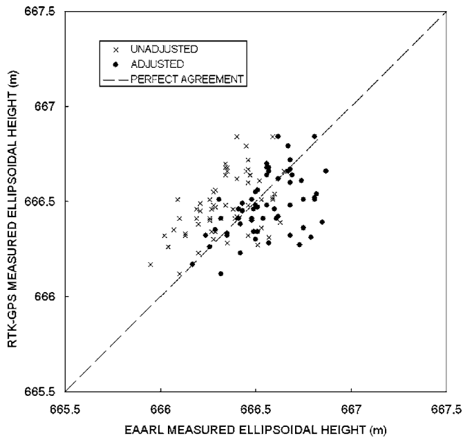
Fig. 3. Graph showing original and block adjusted submerged points in the Cottonwood Ranch reach. EAARL ranging measurements computed with the terrestrial algorithm.
