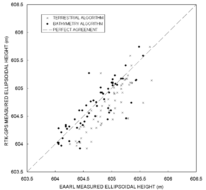
Fig. 4. Comparison of ellipsoidal heights computed with the EAARL terrestrial and bathymetric algorithms with block adjustment in the Rowe Sanctuary study site (depths >0.4 m)
