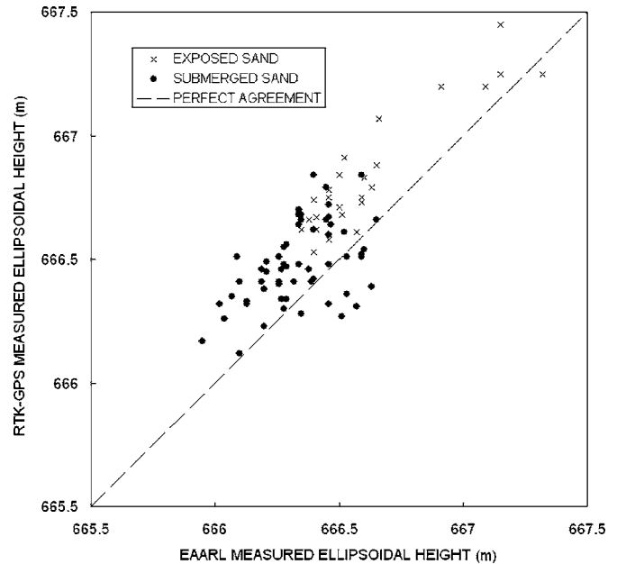
Fig. 2. Graph showing the comparison between ground-truth and unadjusted EAARL heights in the Cottonwood Ranch reach. EAARL range measurements computed with the terrestrial algorithm.
