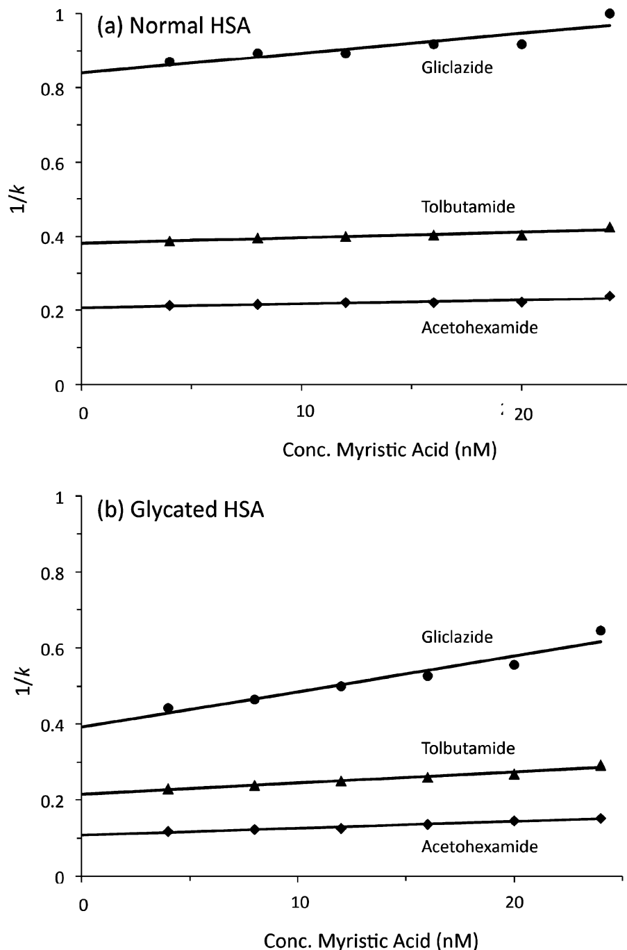
Figure 4. Observed change in the retention factor ( k ) for gliclazide (●), tolbutamide (▲) and acetohexamide (◆) on HPLC columns containing immobilized (a) normal HSA or (b) glycated HSA and in the presence of mobile phases containing various concentrations of myristic acid. All values shown in this figure are the averages of three replicates and had relative standard deviations in the range of \pm 0.1 – 1.6\% .
