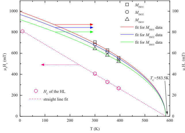
FIG. 5. (Color online) HL coercivity \mu_0 H_C vs T (left axis). Hexagons represent experimental data, the dotted line is an empirical linear best fit. Its extrapolation to \mu_0 H_C = 0 provides an estimate of the HL Curie temperature T_C = 583.5 K. The right axis shows the equilibrium bias field \mu_0 H_B^e vs T for all three isomagnetization set fields. Squares ( M_{ISO1} ), circles ( M_{ISO2} ), and triangles ( M_{ISO3} ) are the experimental data. Lines are single parameter best fits of Eq. (11).
