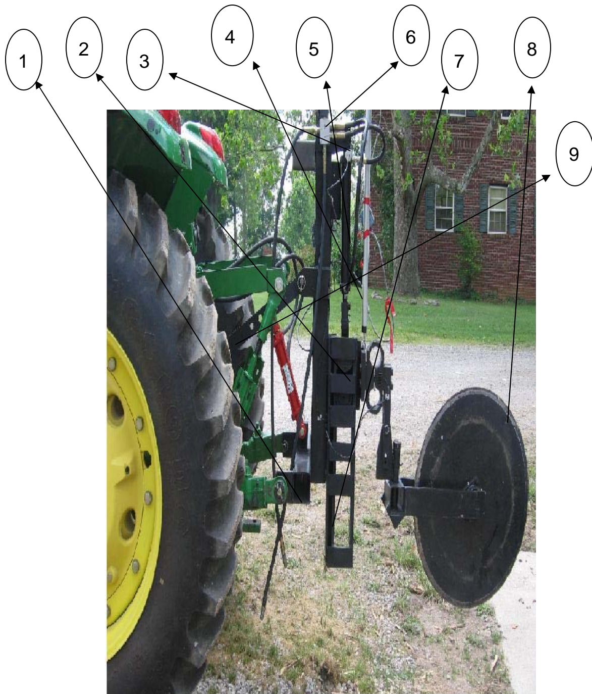
Figure1. Coulters penetrometer mounted on the three-point hitch of a tractor
