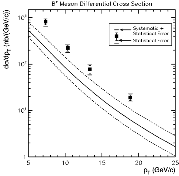
FIG. 3. B^+ meson differential cross measurements compared to the theoretical prediction. The solid curve is the theoretical prediction for m_b = 4.75 \text{GeV}/c^2 , \mu_0 = \sqrt{m_b^2 + p_T^2} , \epsilon_p = 0.006 and f_u = 0.375 . The dashed lines illustrate the changes in the theory once these parameters are varied as explained in the text.
