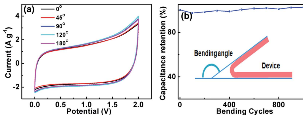
Fig. 5 (a) Cyclic voltammety curves for the supercapacitor at different bending angles from 0 – 180^\circ . (b) Stability of the device during 1000 bending cycles (bending angle: 120^\circ ).
