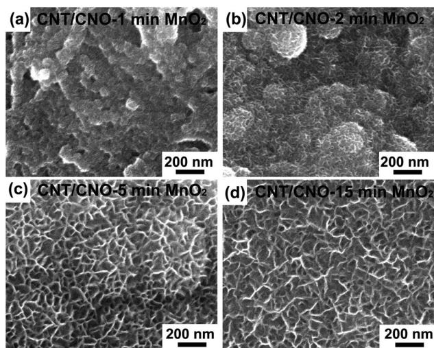
Fig. 2 (a–d) SEM images of CNT/CNO films with MnO 2 deposition for 1, 2, 5, and 15 min.
