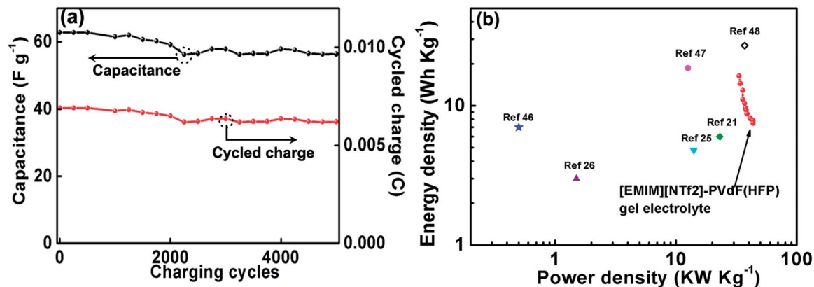
Fig. 6 (a) Retention ratio of the supercapacitor fabricated by 1 min MnO_2/CNT/CNO electrodes and [EMIM][NTf2]-PVdF(HFP) gel electrolyte in 5000 charge-discharge cycles at a current density of 2 mA cm^{-2} . (b) Ragone plots of the supercapacitors using [EMIM][NTf2]-PVdF(HFP) gel electrolytes.
