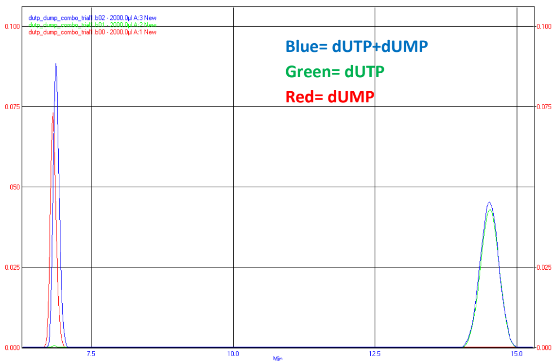
Figure 2.5: Elution profiles of dUMP and dUTP. Traces represent 2 mL injections of 10 \mu M (20 nanomoles) dUMP (red), dUTP (green) or both dUMP and dUTP (blue). Nucleotides were in 10 mM bicine, pH 8.0.
