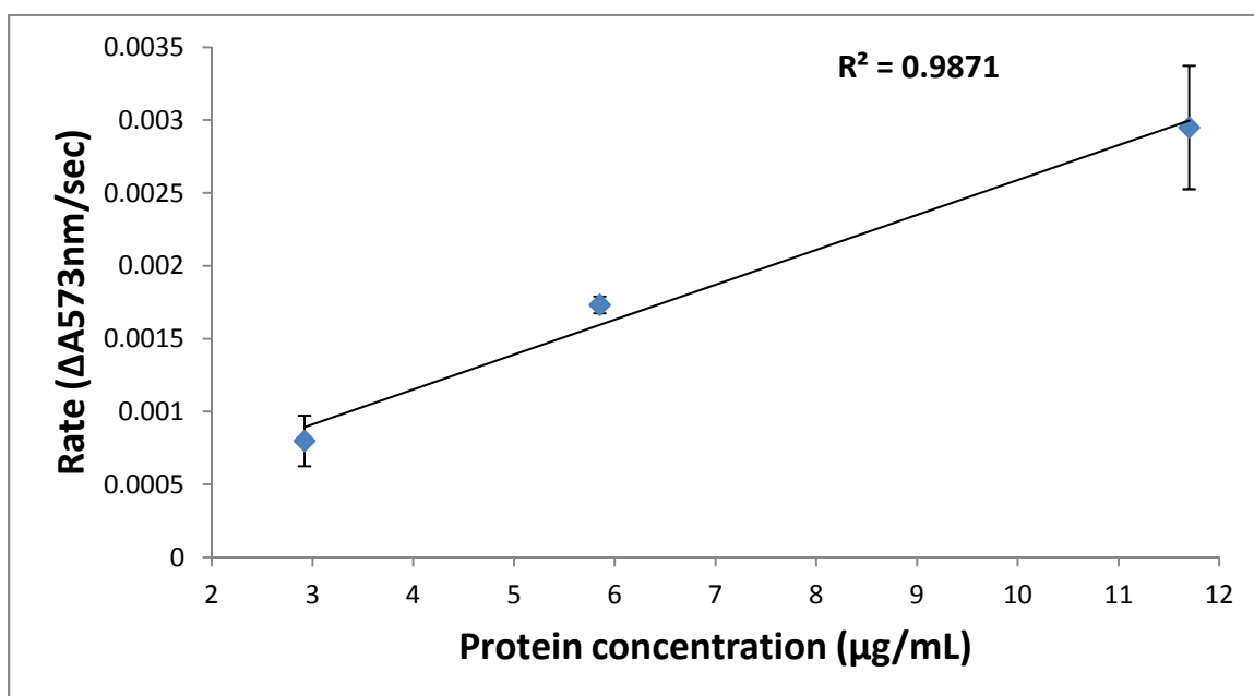
Figure 3.4: Range of linearity for the activity of the core dUTPase. Protein concentrations of 2.92 \mu g/mL, 5.85 \mu g/mL, and 11.7 \mu g/mL were used to determine the linear portion of the activity curve at 10 \mu M dUTP.
