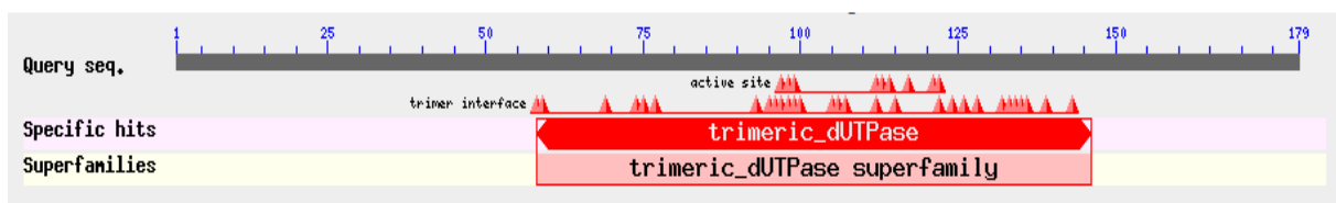
Figure 3.2: Basic Local Alignment Search Tool (BLAST) of full-length D. discoideum dUTPase. This figure represents the protein sequence annotation of dUTPase, revealing the location of trimer interface and active site residues. BLAST results can be located in the Appendix Section 5.5.
