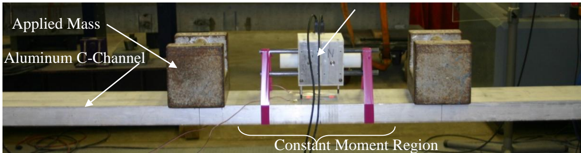
Figure 4.6 Channel Loaded
