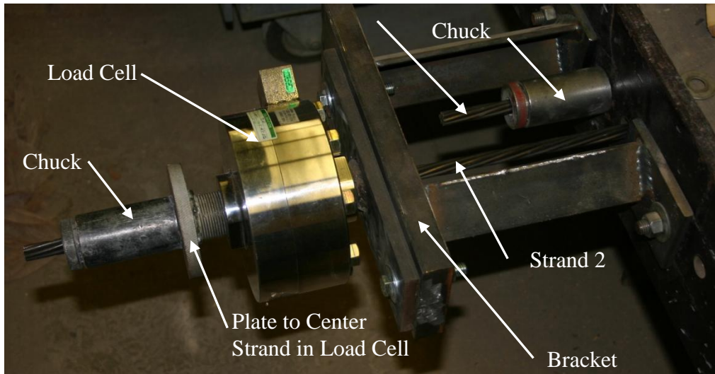
Figure 3.6 Load-Cell Bracket
