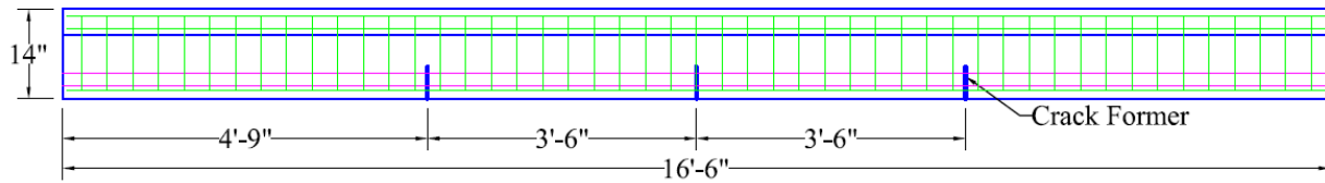
Figure 3.10 Locations of Crack Formers
