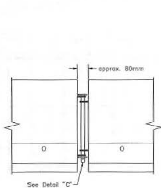
Connection Detail
