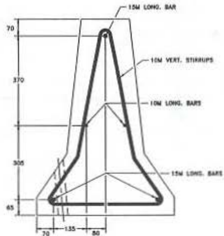
INTERIOR STIRRUP
