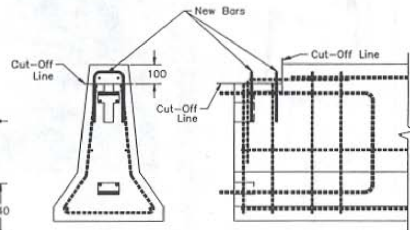
Rebar Details
