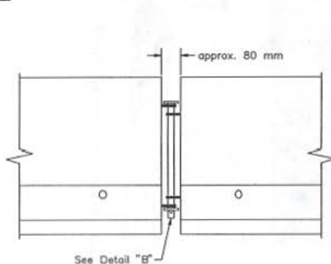
Connection Detail
