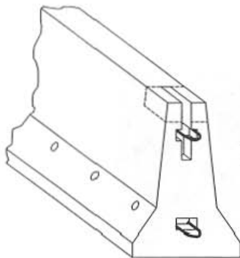
Retrofit Step One Cut away concrete along dotted line (avoid rebar).
