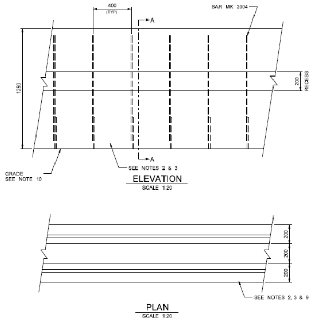
Figure 4: plan and elevation views of the median barrier end section
