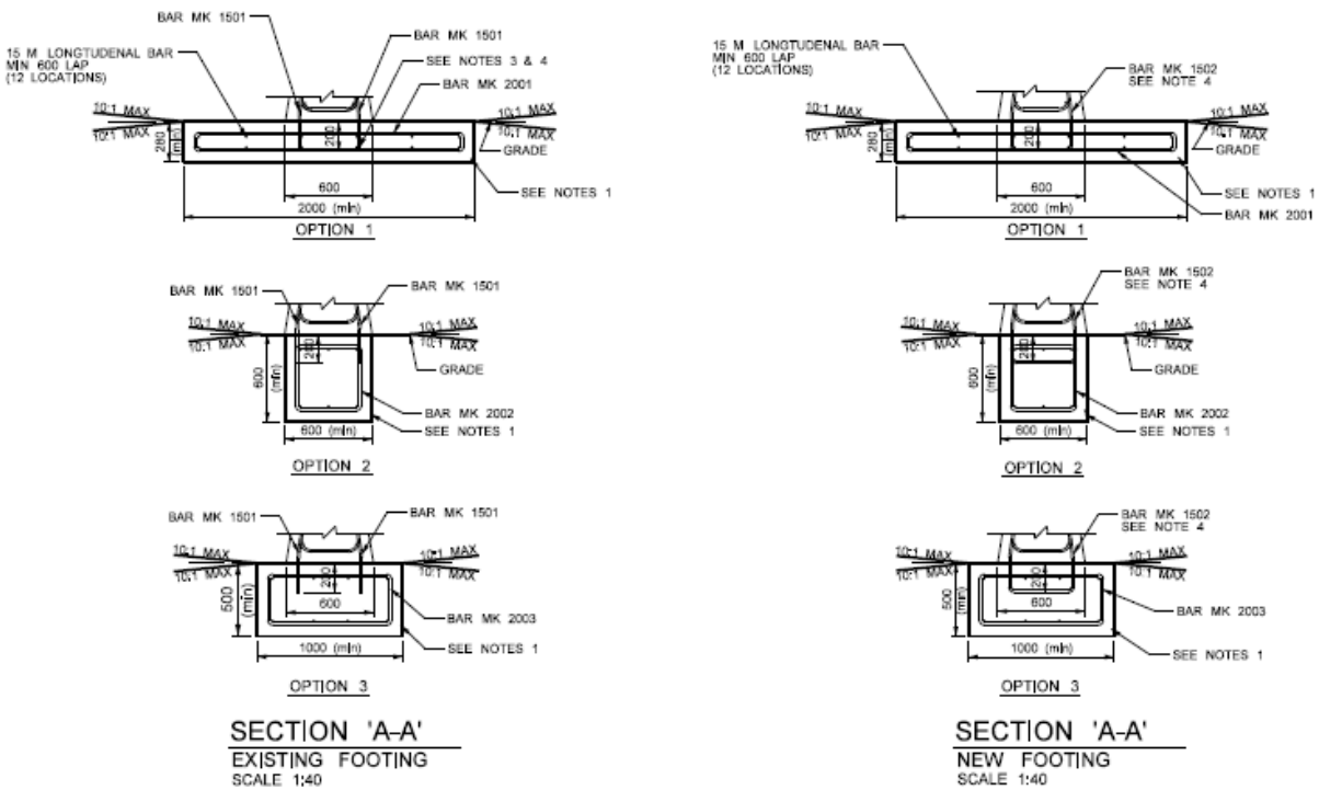
Figure 6: Cross section views of median barrier footing options
