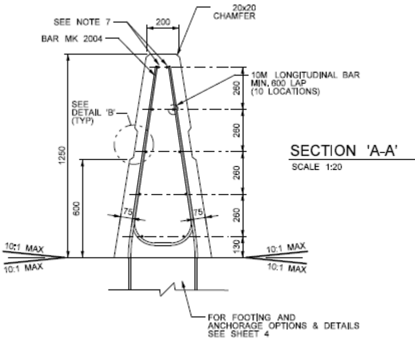
Figure 6: Cross section views of median barrier footing options
