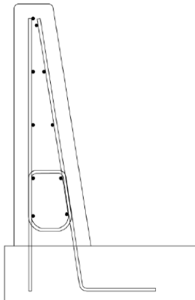
Figure 1: General configuration of Manitoba Constrained-Width Tall Wall bridge rail
