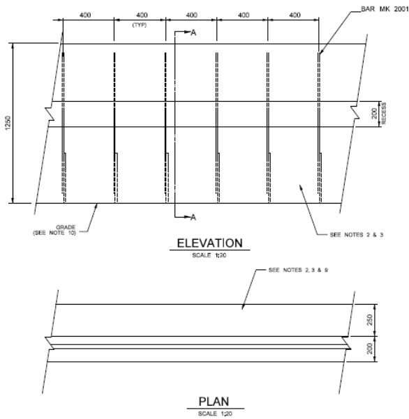
Figure 8: plan and elevation views of the roadside barrier end section
