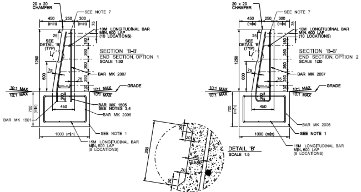
Figure 10: Cross section views of the end section roadside barrier, footings and anchorage options
