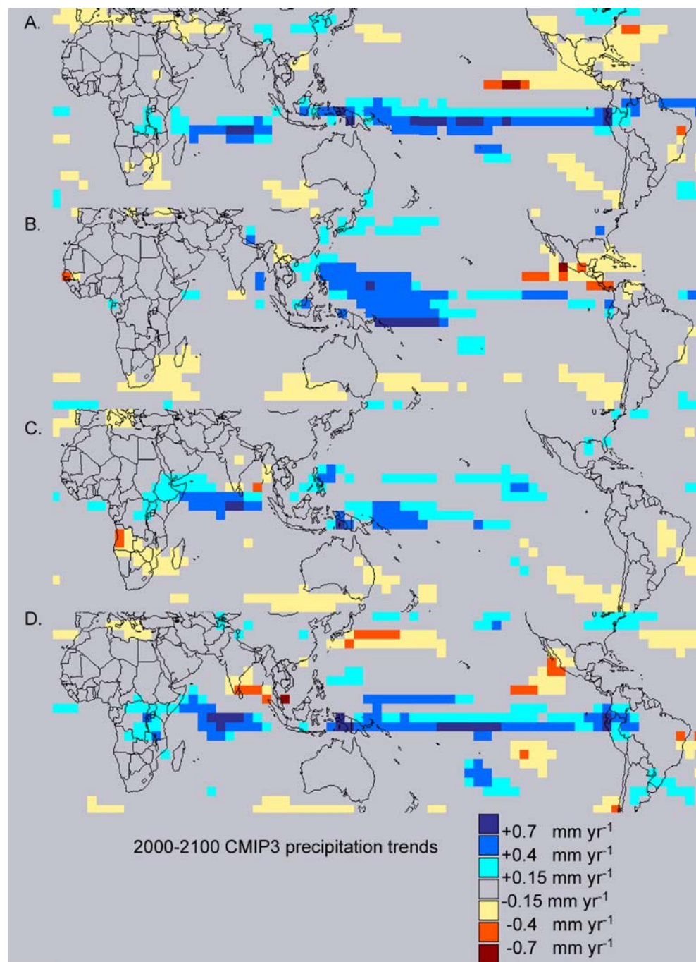
Fig. 4 Predicted precipitation changes for the 21st century, based on a large set of climate change scenarios (See Table 2). The outputs from these simulations were averaged for each quarter (March-April-May: A, June-July-August: B, September-October-November: C, December-January-February: D). Trends for the time period 2000–2100 were then calculated and plotted. The model simulation shows substantial increases in rainfall over the oceans
