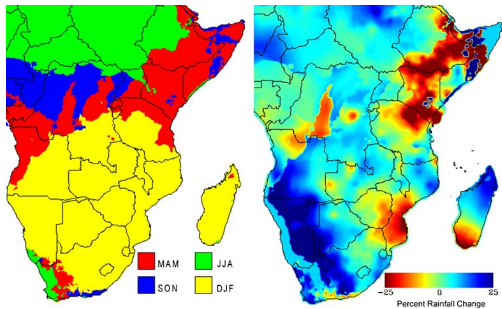
Fig. 7 Main growing quarters (left panel: MAM, JJA, SON, DJF) and rainfall projections, expressed as % change for 2050 for these quarters (right panel) as described by the hybrid dynamic-statistical precipitation reformulations for eastern and southern Africa. They are based on 21st century projections of central Indian Ocean [0–15°S, 60–90°E] precipitation and global precipitation 1st principal components (IO and PC1, respectively). Changes in rainfall were obtained by multiplying the IO and PC1 regression parameters by the seasonally appropriate changes shown in Fig. 5
